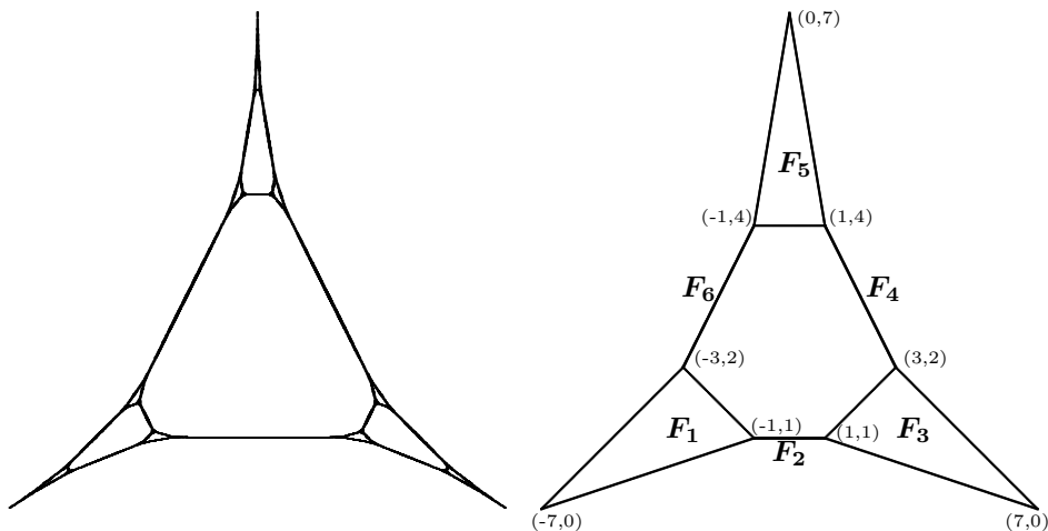
FIGURE 3. The hexagasket in harmonic coordinates and its first approximation.
