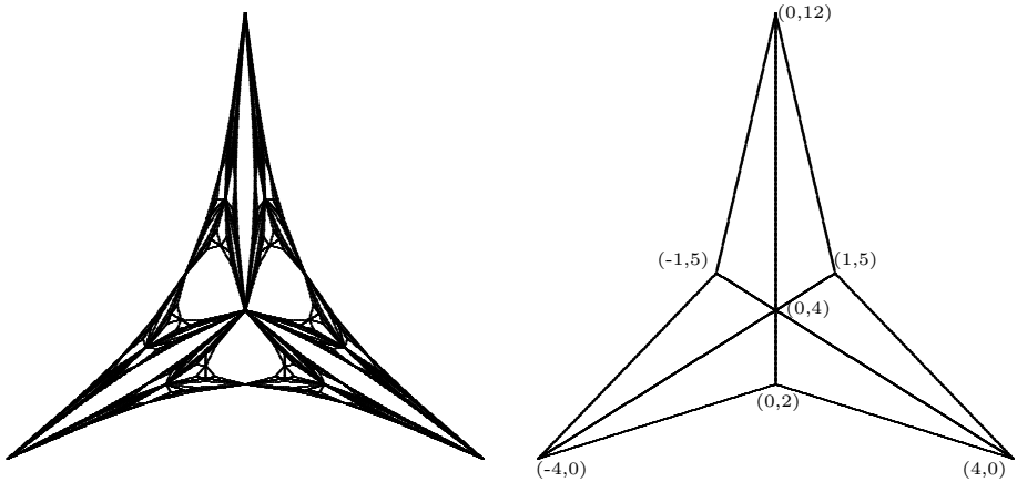
FIGURE 6. A non regular post-critically infinite fractal and its first approximation.
