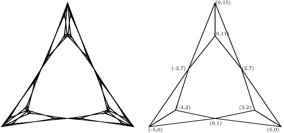
FIGURE 5. A regular post-critically infinite fractal and its first approximation.
