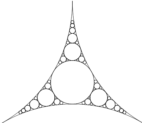
FIGURE 2. The residue set of the Apollonian packing.
